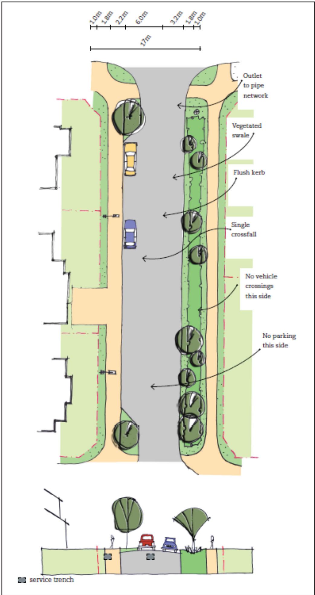
Figure 9 - Road Typology F - Swale Street
